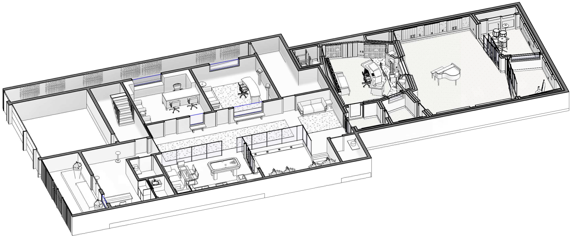
AXONOMETRIC VIEW - COMPLETE BUILDING
